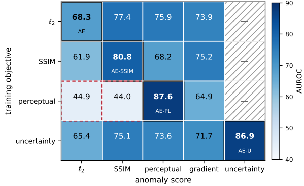
Figure 1: The objective \times score grid on RSNA, AUROC over three seeds. Boxed cells are the diagonal and name the published method they instantiate; red dashed cells are below chance; hatched cells are undefined, the uncertainty score needing a variance only the heteroscedastic objective emits (Section 3 supplies a proxy). The other two datasets are in Section B.
